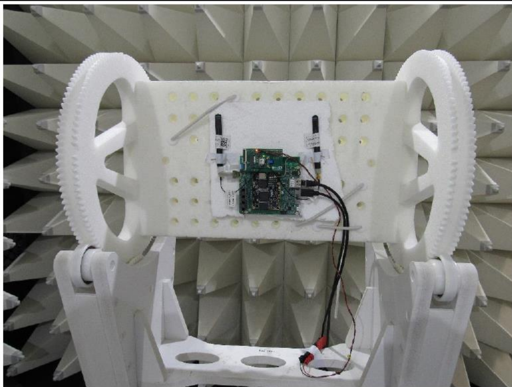
EUT set up above 1 GHz
