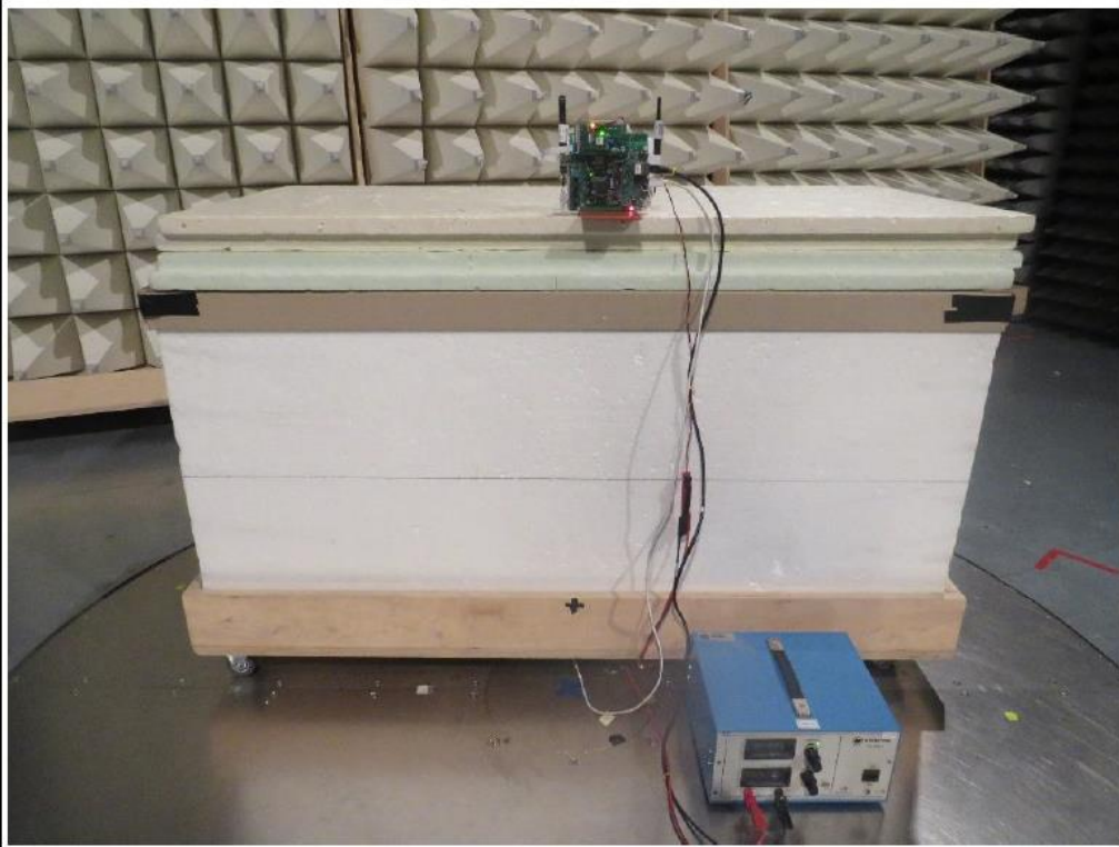
EUT set up below 1 GHz
