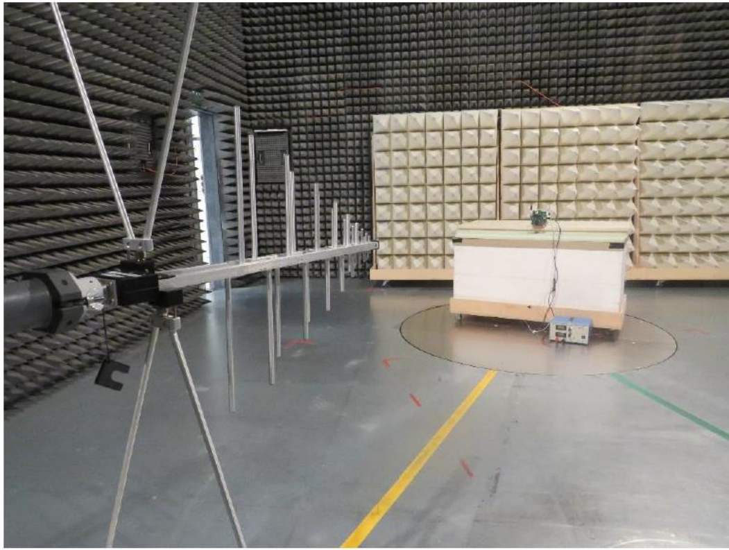
Test set up below 1 GHz
