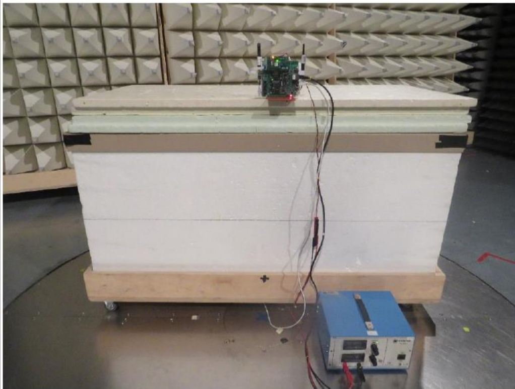
EUT set up below 1 GHz
