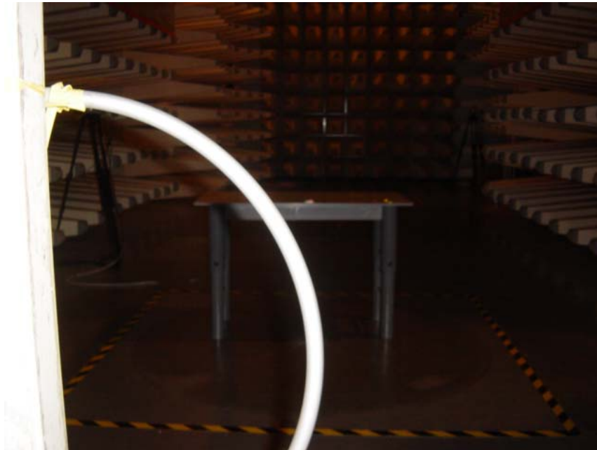
Set-up for Radiation Emission (Transceiver)
