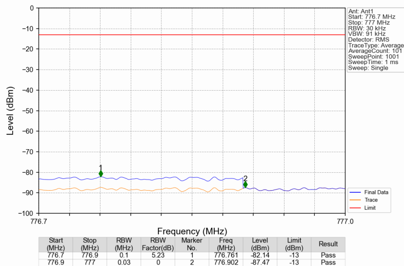
Band13_748.5MHz_AWGN_SISO_Ant1_NTNV_AGC+3
