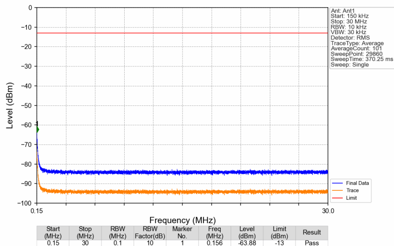
Band13_753.5MHz_AWGN_SISO_Ant1_NTNV
