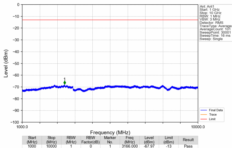
Band13_748.5MHz_AWGN_SISO_Ant1_NTNV
