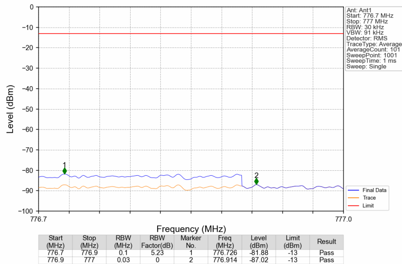
Band13_748.5MHz_AWGN_SISO_Ant1_NTNV_AGC
