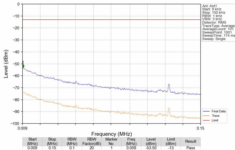
Band13_753.5MHz_AWGN_SISO_Ant1_NTNV
