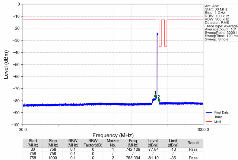
Band13_753.5MHz_AWGN_SISO_Ant1_NTNV
