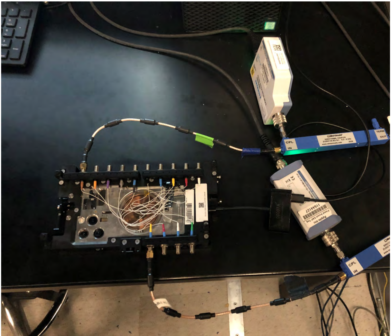
Figure C-3 UXM Conducted power test measurement setup dual port
