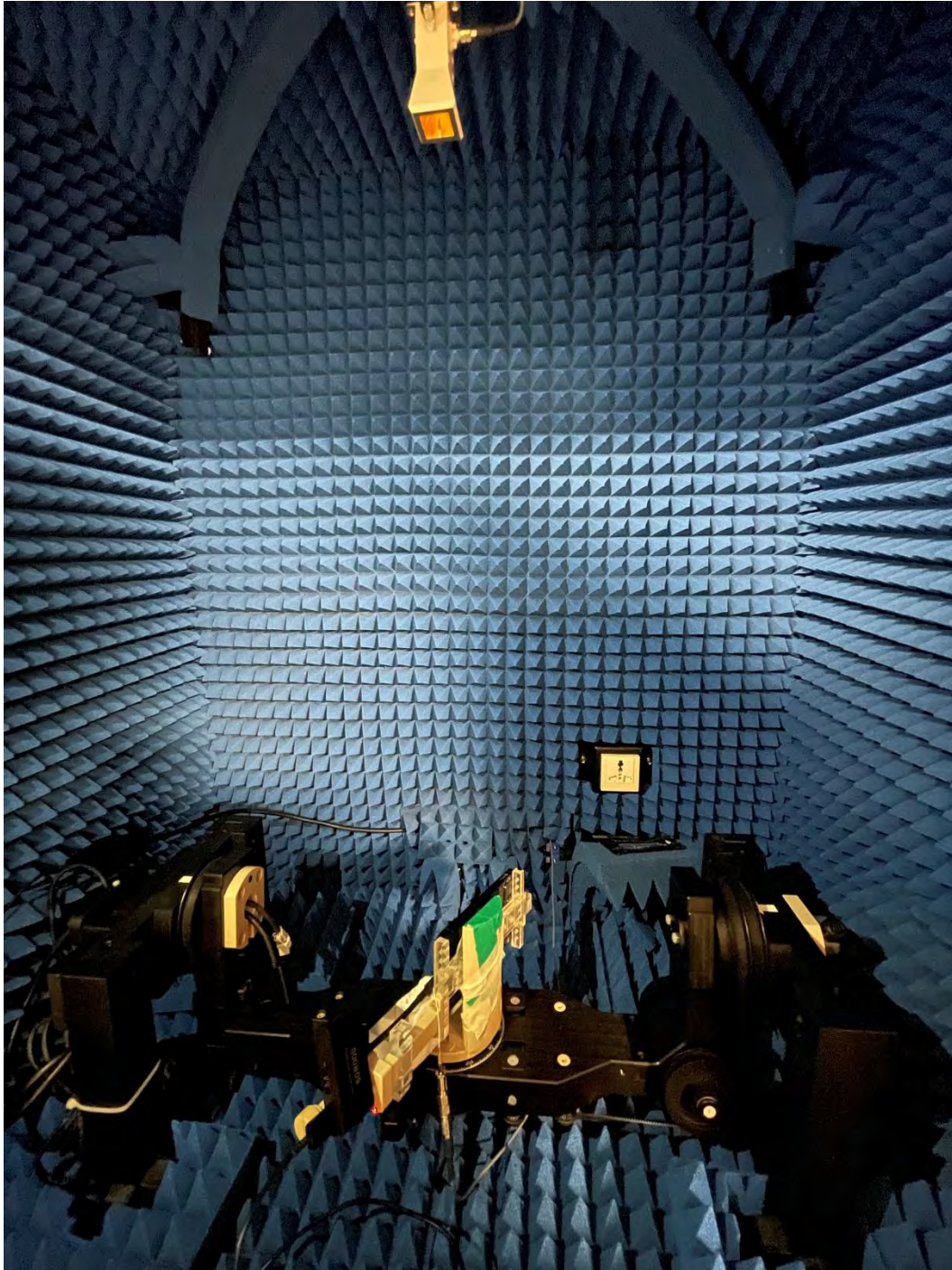
Figure C-5 Radiated power mmW test measurement setup
