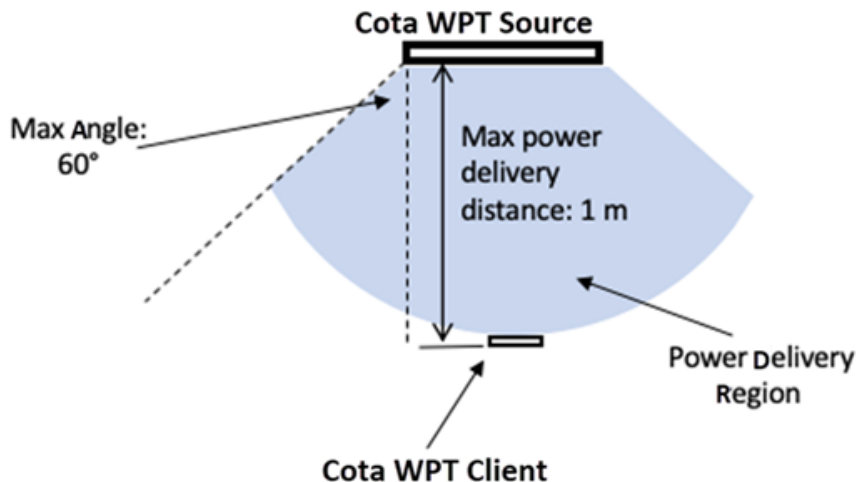
Figure 2 Cota Wireless Power Transfer System Power Delivery Region
