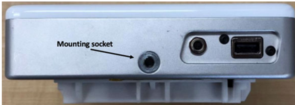
Figure 1 Cota Wireless Power Transfer Client Mounting Socket
